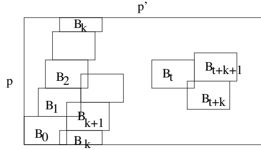
Figure 1: Covering the torus grid with rectangles
